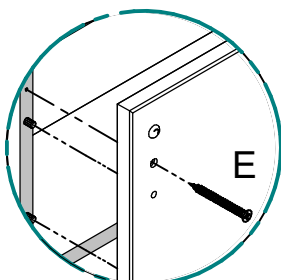
Detail 6
